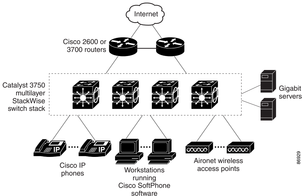
Figure 1-6 Catalyst 3750 Stack in a Collapsed Backbone Configuration
