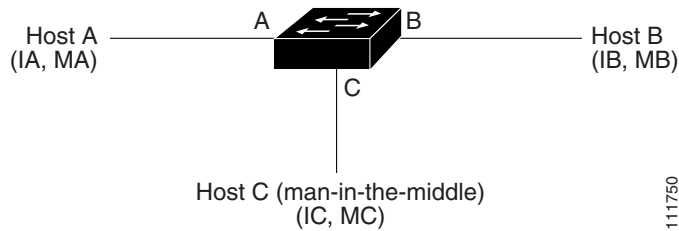
Figure 24-1 ARP Cache Poisoning
