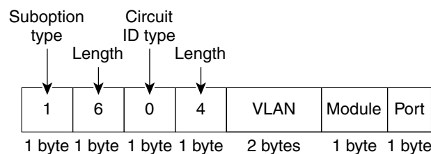
Figure 23-2 Suboption Packet Formats
