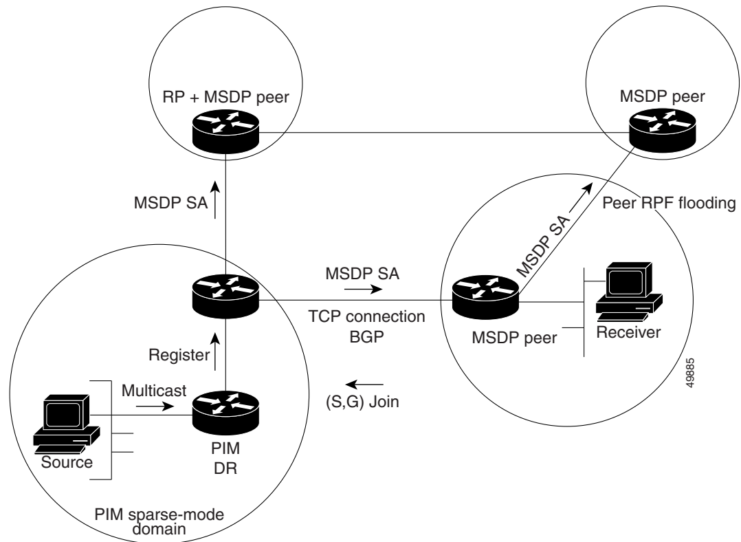
Figure 4-1 MSDP Running Between RP Peers
