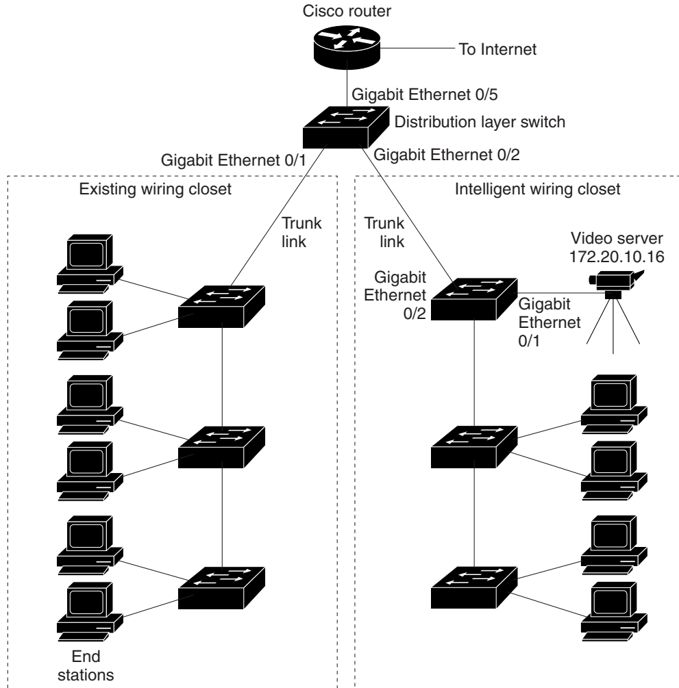
Figure 30-11 QoS Configuration Example Network
