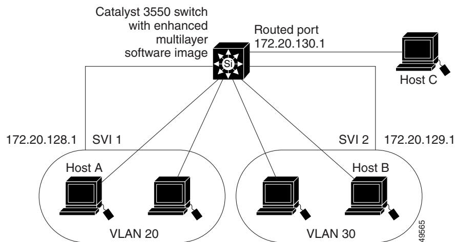
Figure 26-1 Fallback Bridging Network Example
