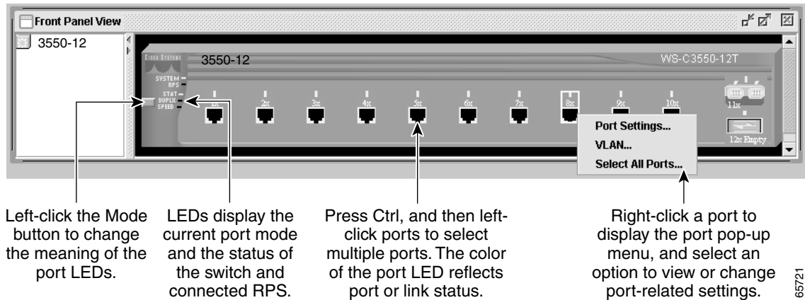
Figure 3-2 Front Panel View from a Standalone Switch
