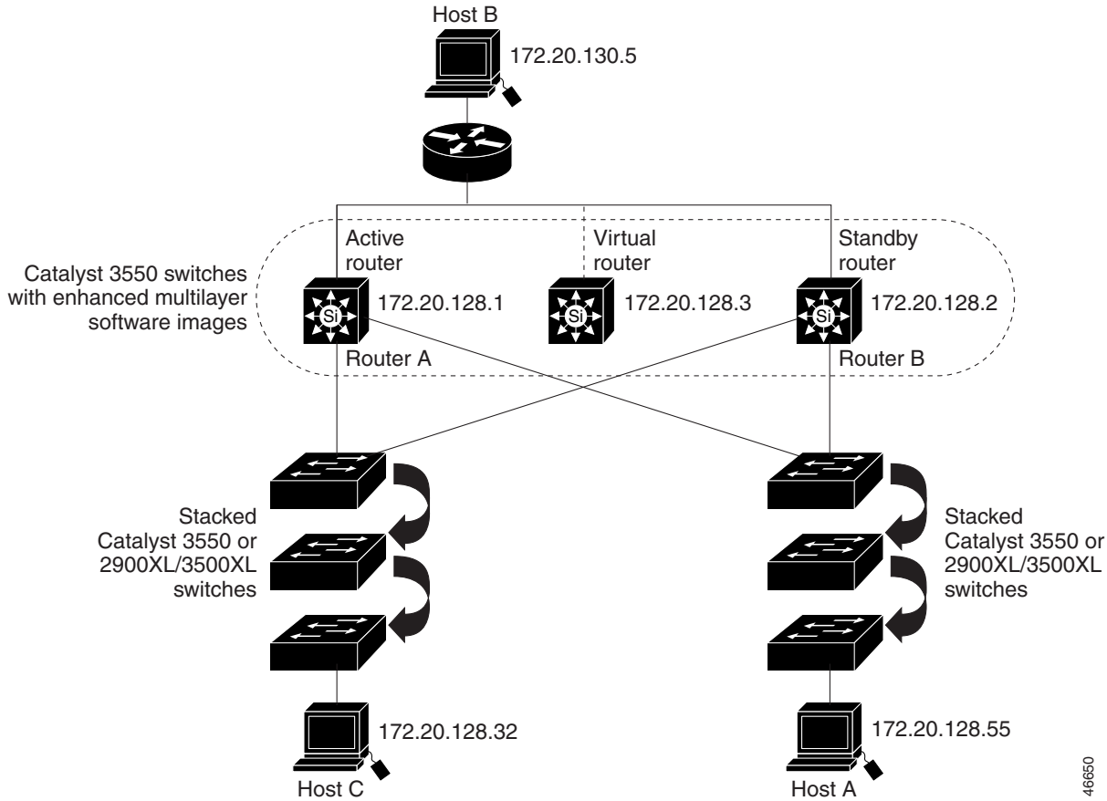
Figure 23-1 Typical HSRP Configuration
