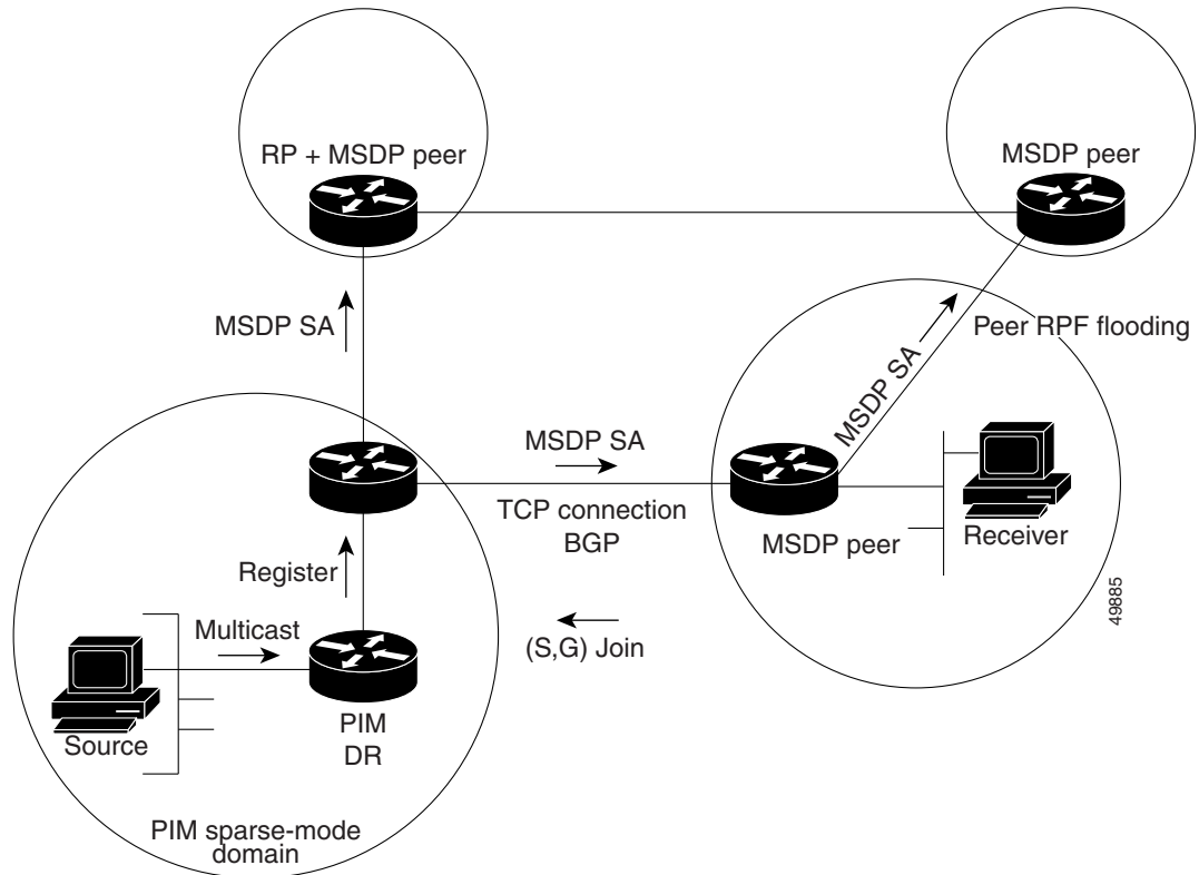
Figure 23-1 MSDP Running Between RP Peers
