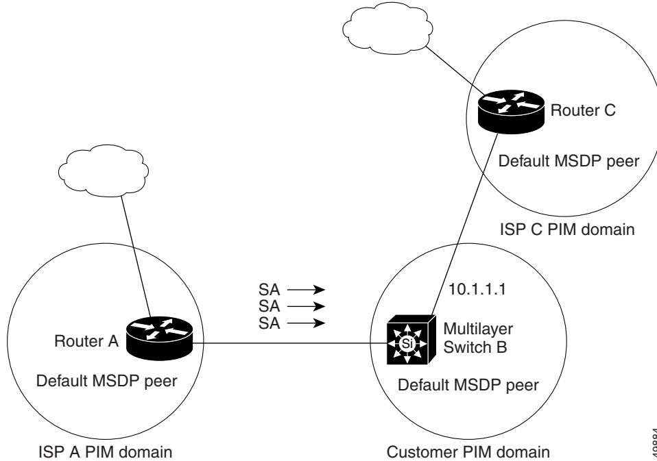
Figure 23-2 Default MSDP Peer Network
