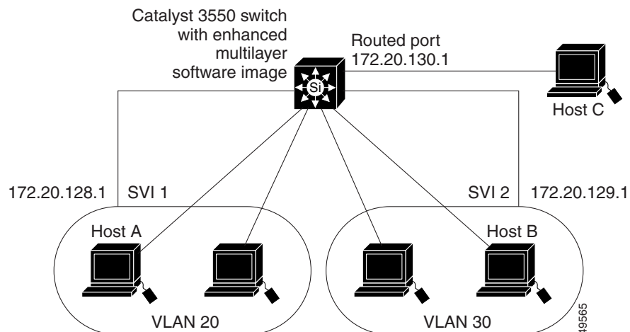
Figure 34-1 Fallback Bridging Network Example
