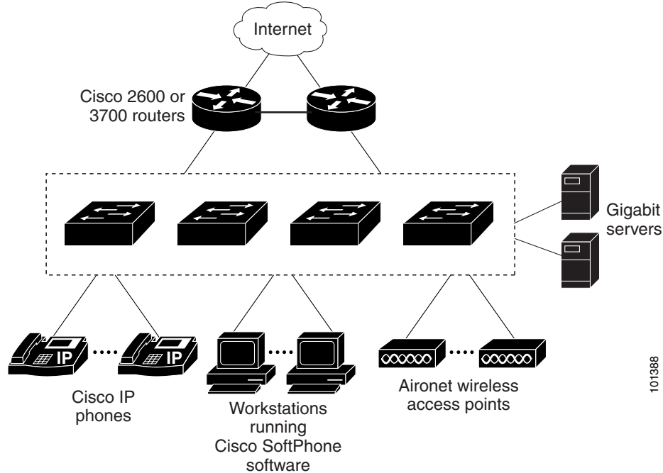
Figure 1-3 Catalyst 2970 Switches in a Collapsed Backbone Configuration
