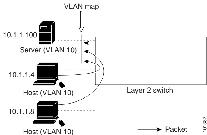
Figure 27-4 Deny Access to a Server on Another a VLAN
