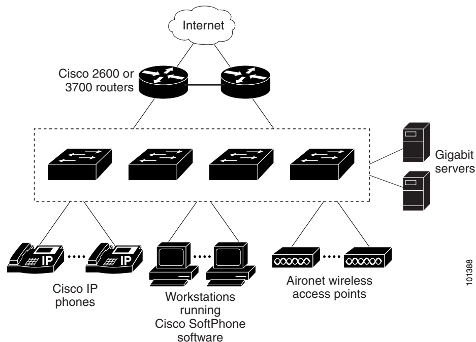
Figure 1-3 Catalyst 2970 Switches in a Collapsed Backbone Configuration
