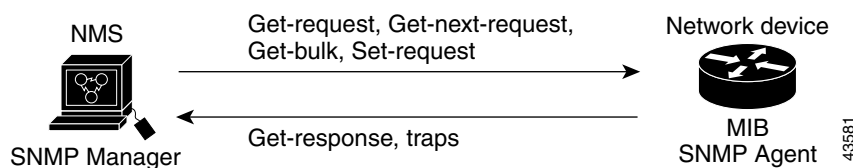
Figure 25-1 SNMP Network
