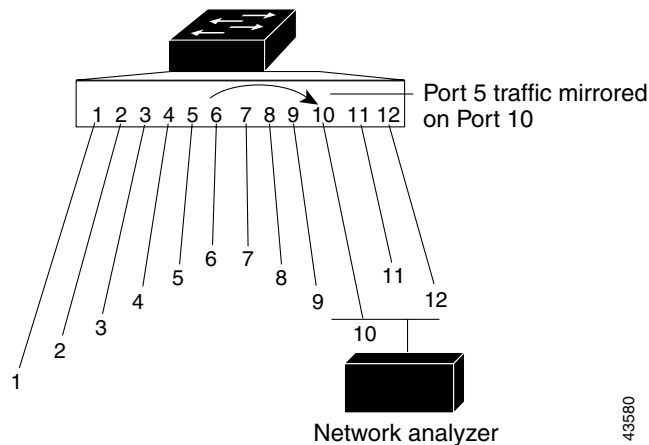
Figure 20-1 Example of Local SPAN Configuration on a Single Switch
