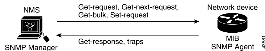
Figure 23-1 SNMP Network
