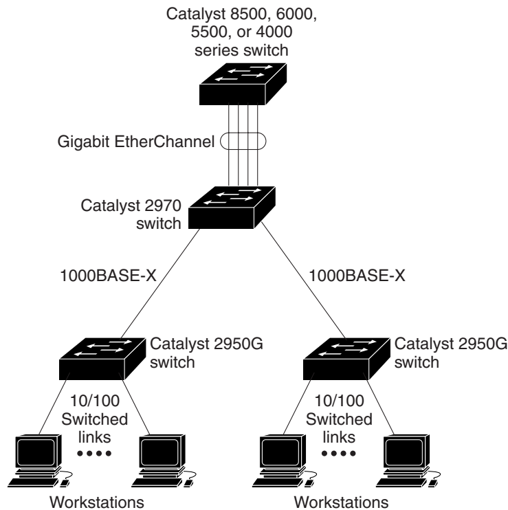
Figure 26-1 Typical EtherChannel Configuration
