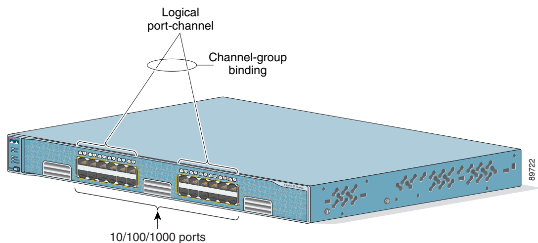
Figure 26-2 Relationship of Physical Ports, Logical Port Channels, and Channel Groups
