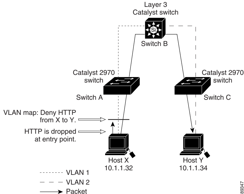
Figure 24-3 Wiring Closet Configuration
