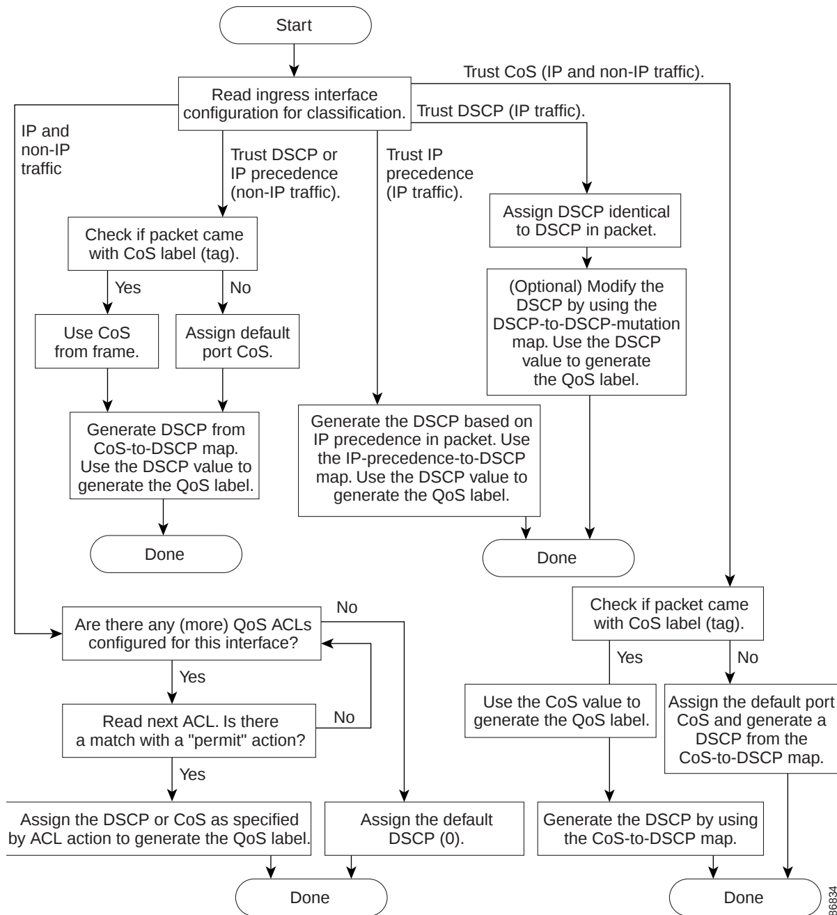
Figure 1-3 Classification Flowchart
