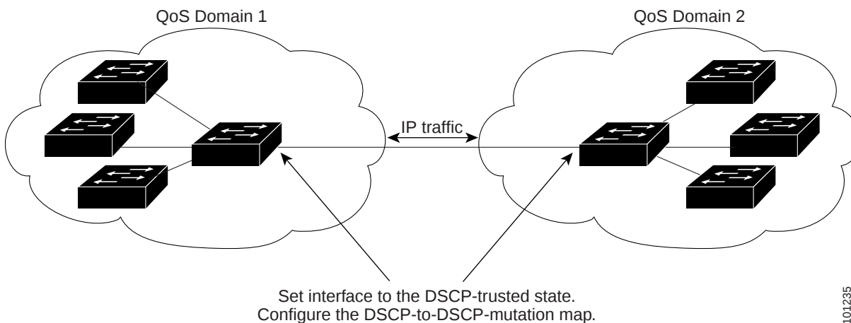
Figure 1-11 DSCP-Trusted State on a Port Bordering Another QoS Domain
