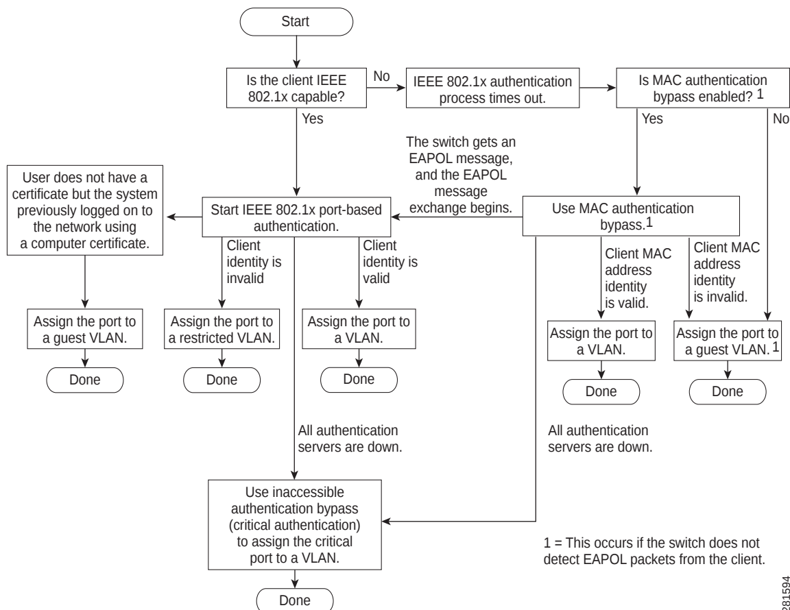
Figure 1-2 Authentication Flowchart
