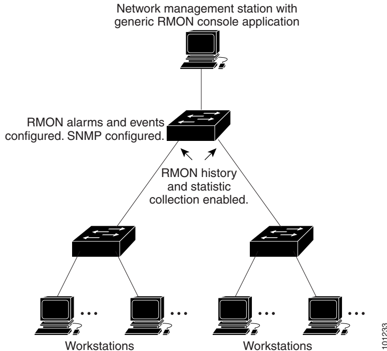
Figure 27-1 Remote Monitoring Example
