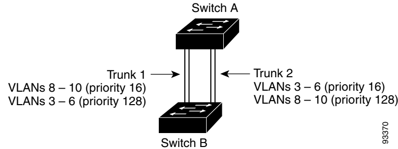
Figure 12-2 Load Sharing by Using STP Port Priorities
