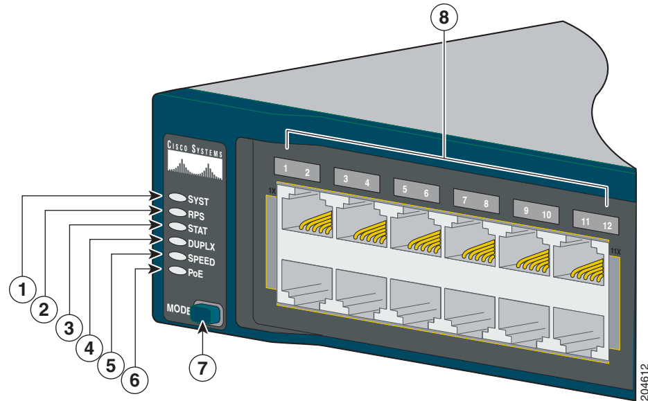
Figure 1-23 Catalyst 2960 Switch LEDs
