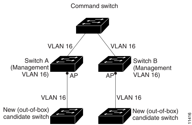
Figure 7-6 Discovery of Newly Installed Switches in the Same Management VLAN
