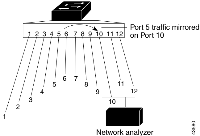
Figure 20-1 Example SPAN Configuration
