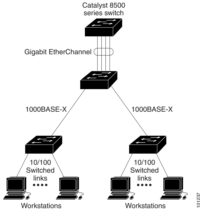
Figure 25-1 Typical EtherChannel Configuration
