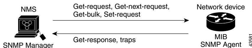
Figure 24-1 SNMP Network
