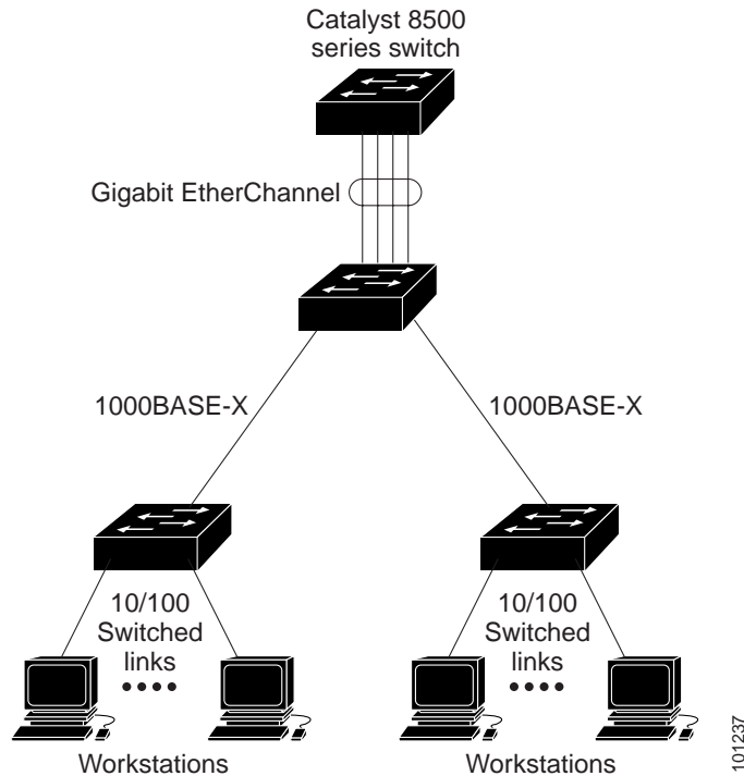
Figure 26-1 Typical EtherChannel Configuration
