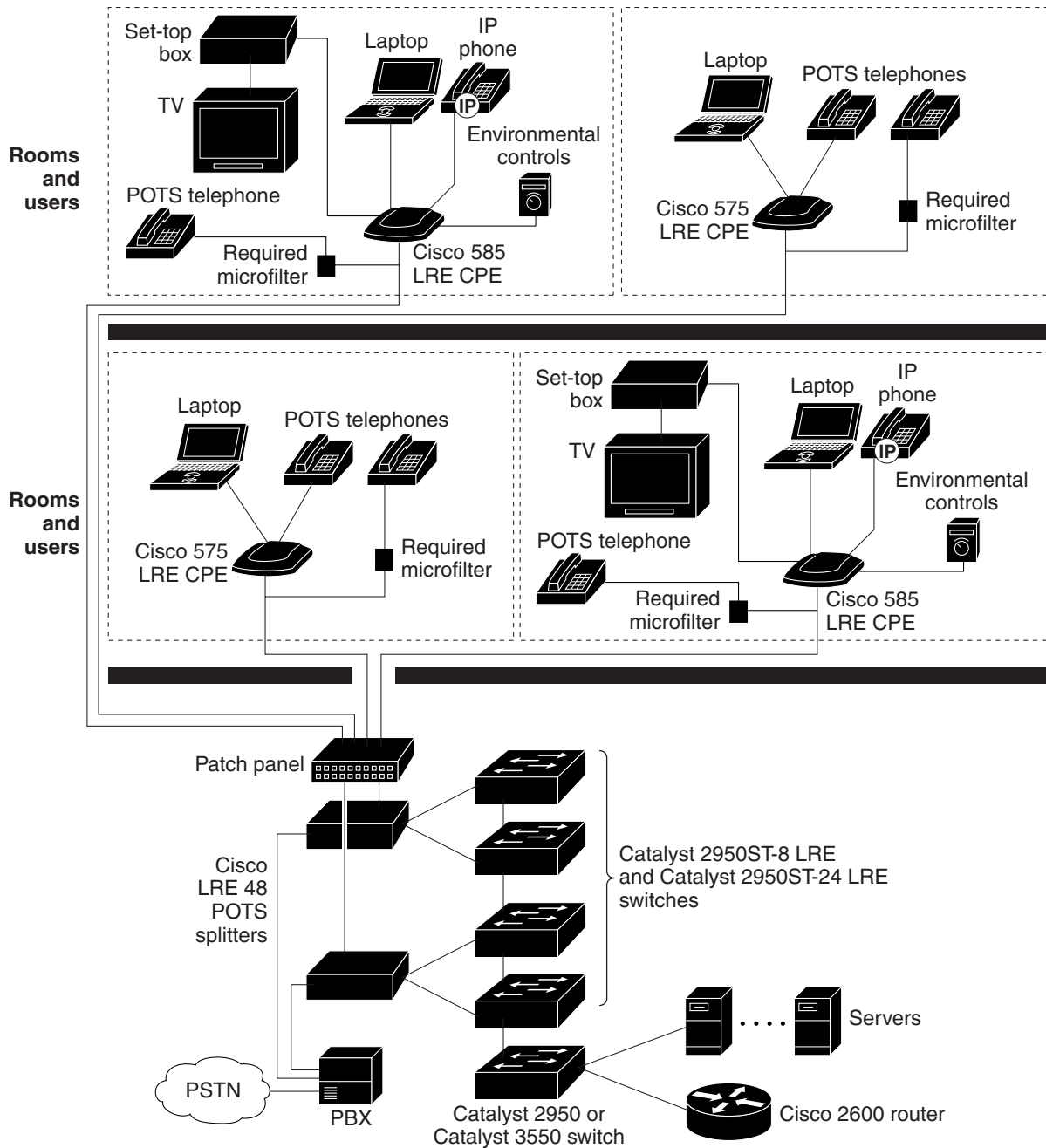
Figure 1-5 Hotel Network Configuration
