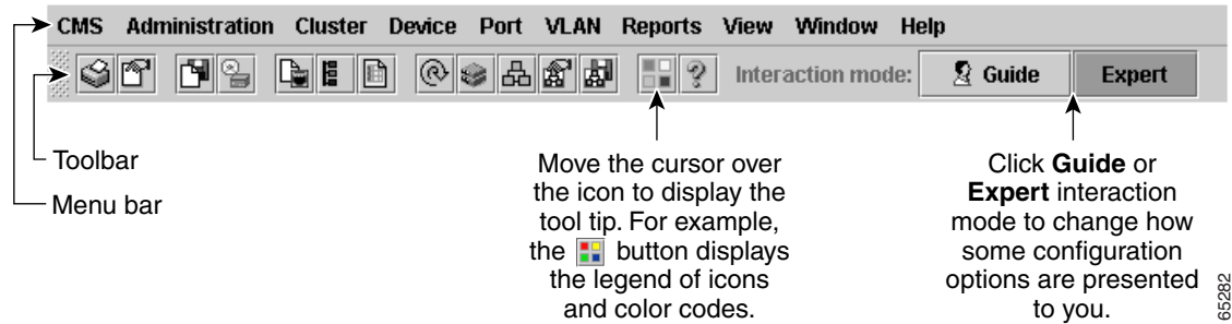
Figure 2-1 CMS Features
