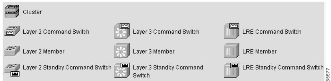
Figure 2-4 Cluster-Tree Icons
