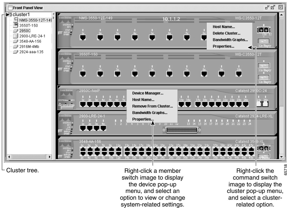
Figure 2-3 Front Panel View from a Command Switch
