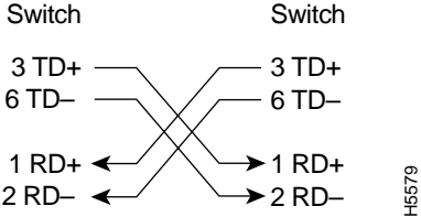
Figure B-3 Straight-Through Cable Schematic
