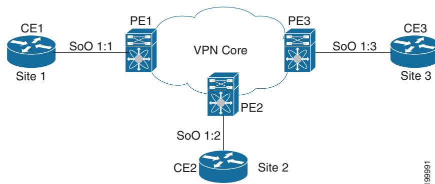
Figure 22-3 Sample MPLS Layer3 Network
