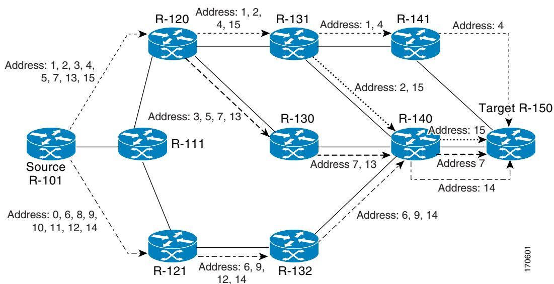
Figure 36-1 MPLS LSP Multipath Tree Trace Path Discovery in a Sample Network
