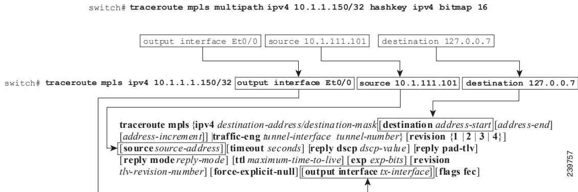
Figure 36-2 Mapping of traceroute mpls multipath Command Output to a traceroute mpls Command
