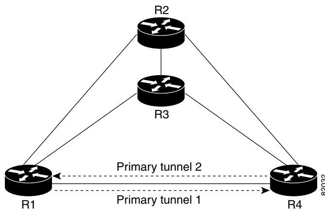
Figure 20-6 Overloaded Link
