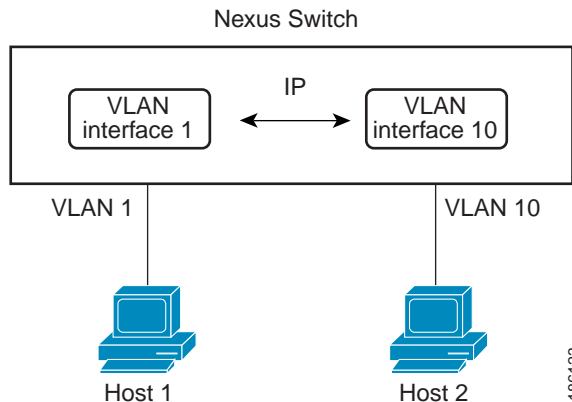
Figure 4-2 Connecting Two VLANs with VLAN interfaces
