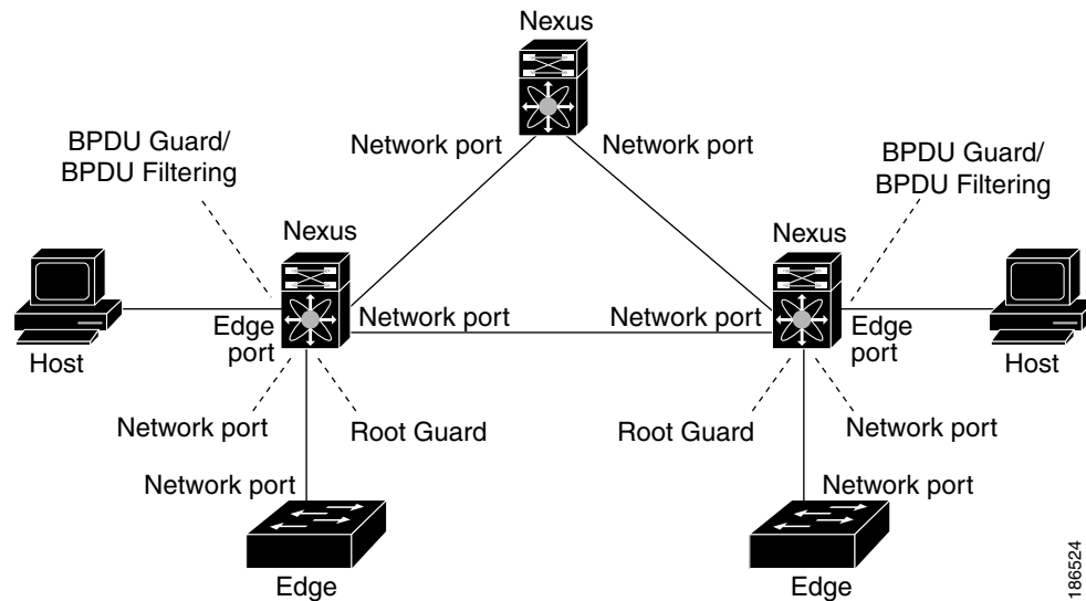
Figure 7-5 Network with STP Extensions Correctly Deployed
