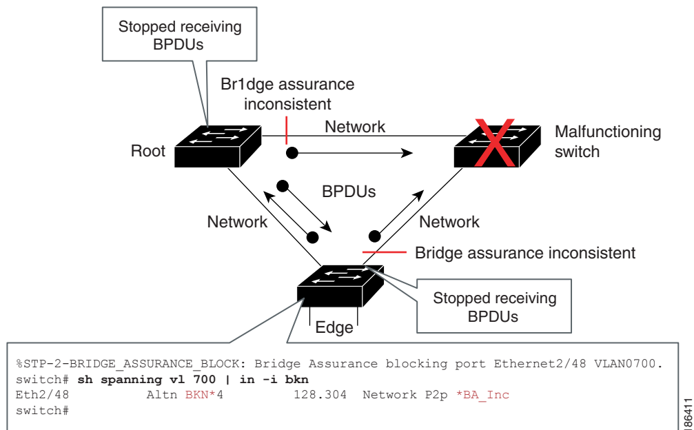
Figure 7-4 Network Problem Averted with Bridge Assurance Enabled
