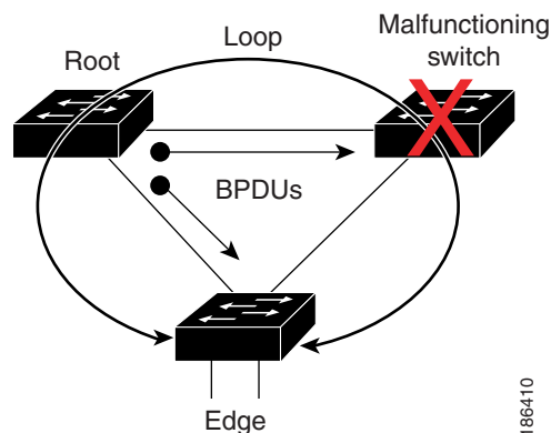
Figure 7-2 Network Problem without Running Bridge Assurance
