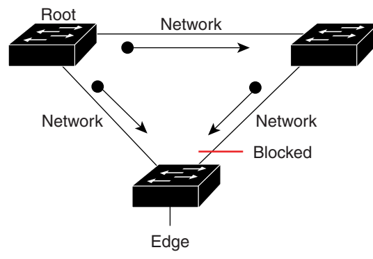
Figure 7-2 Network Problem without Running Bridge Assurance
