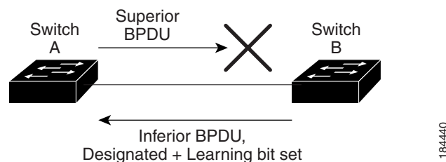
Figure 5-7 Detecting Unidirectional Link Failure
