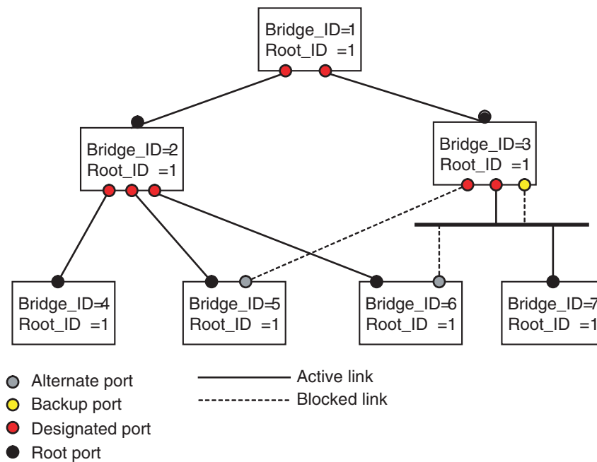
Figure 5-5 Sample Topology Demonstrating Port Roles
