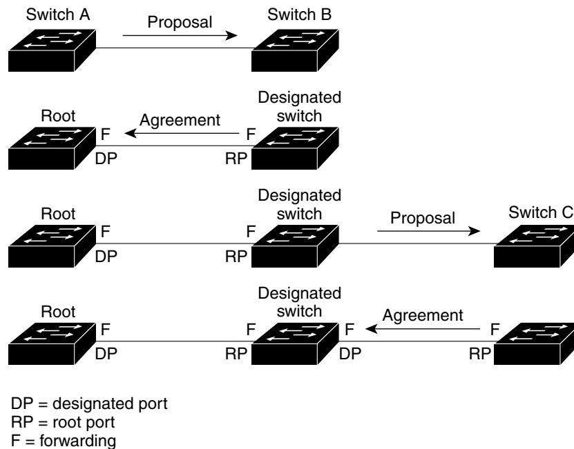
Figure 5-4 Proposal and Agreement Handshaking for Rapid Convergence
