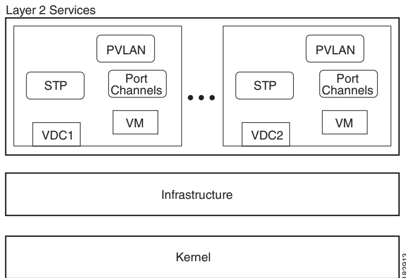
Figure 5-8 Separate STP in each VDC
