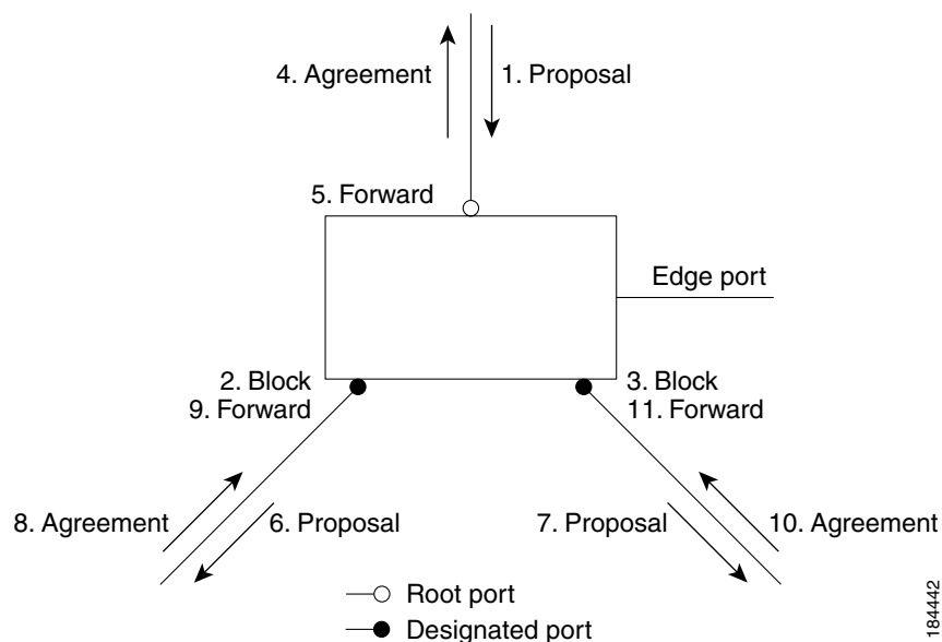
Figure 5-6 Sequence of Events During Rapid Convergence
