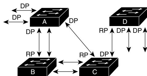
Figure 5-2 Spanning Tree Topology
