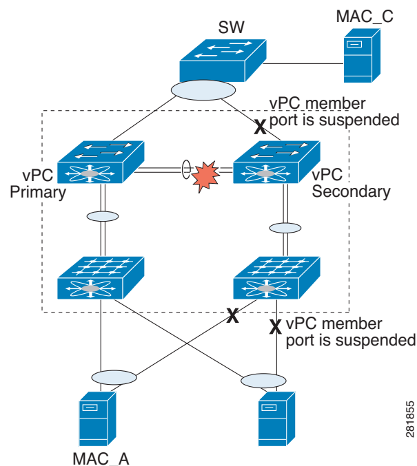
Figure 2-2 vPC Response to a Peer Link Failure
