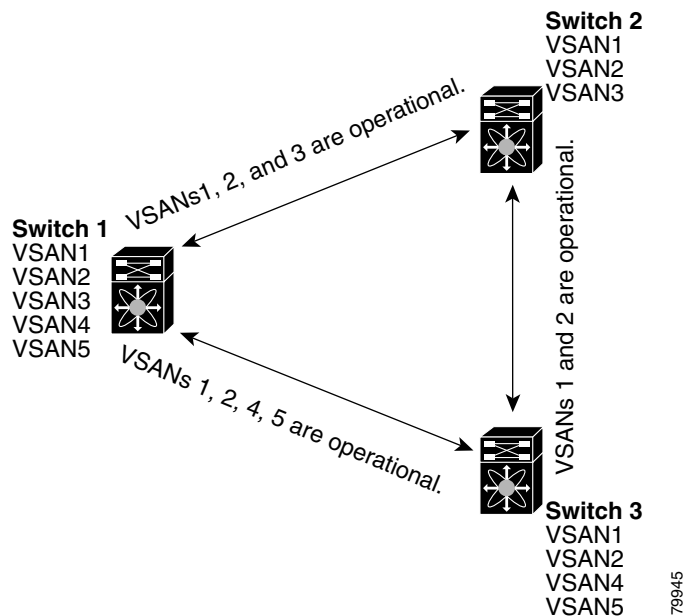
Figure 34-4 Default Allowed-Active VSAN Configuration
