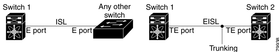
Figure 34-1 VSAN Trunking
