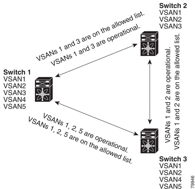
Figure 34-5 Operational and Allowed VSAN Configuration
