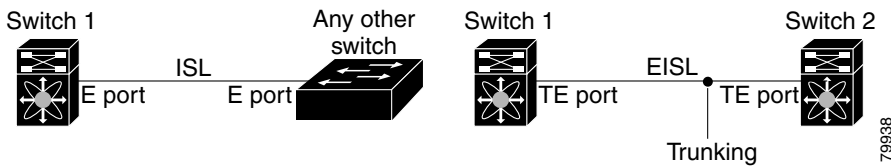
Figure 35-1 VSAN Trunking Only
