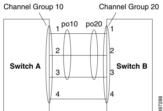
Figure 35-7 Autocreating Channel Groups
