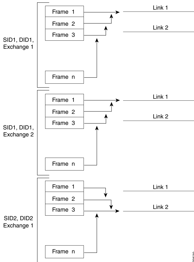
Figure 35-3 SID1, DID1, and Flow-Based Load Balancing
