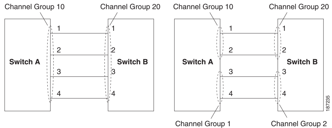
Figure 35-5 Valid SAN Port Channel Configurations
