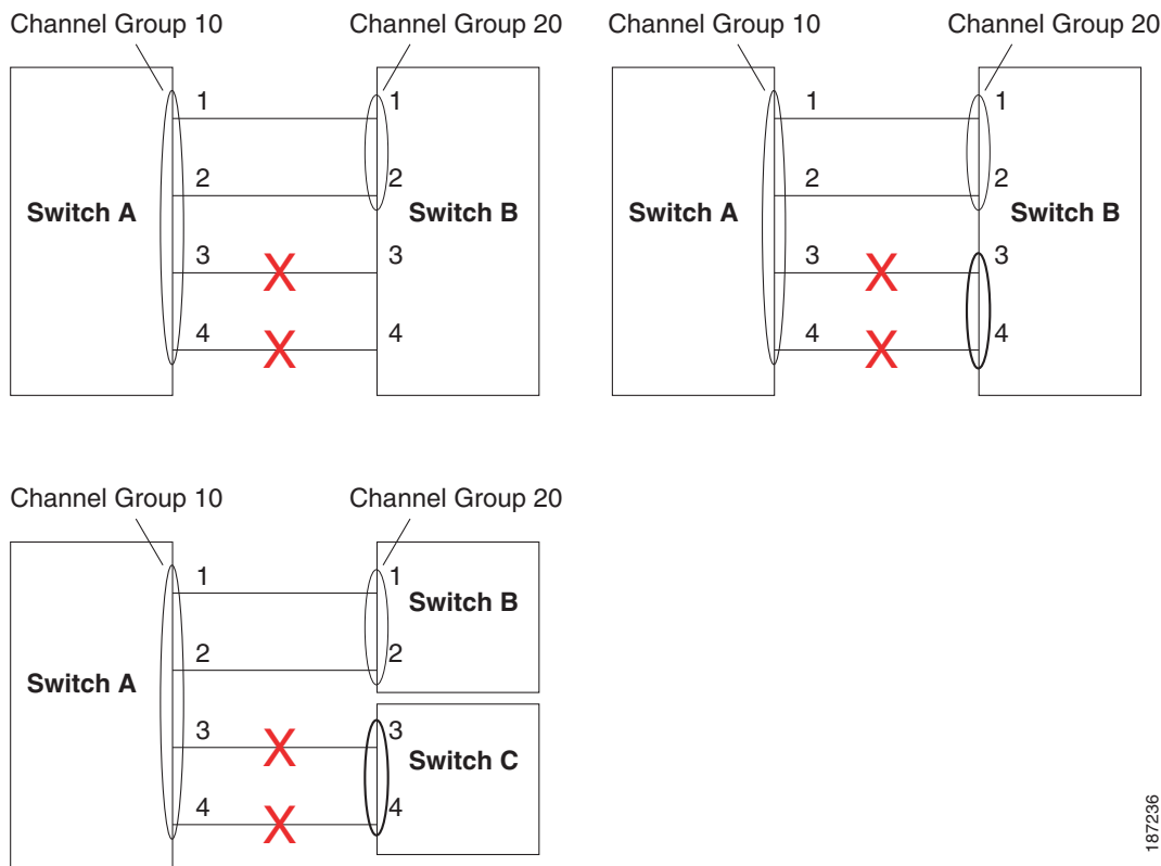
Figure 35-6 Misconfigured Configurations
