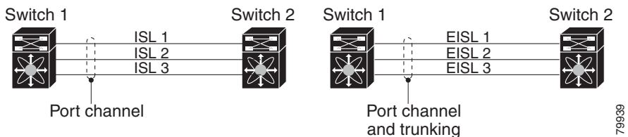
Figure 35-2 Port Channels and VSAN Trunking
