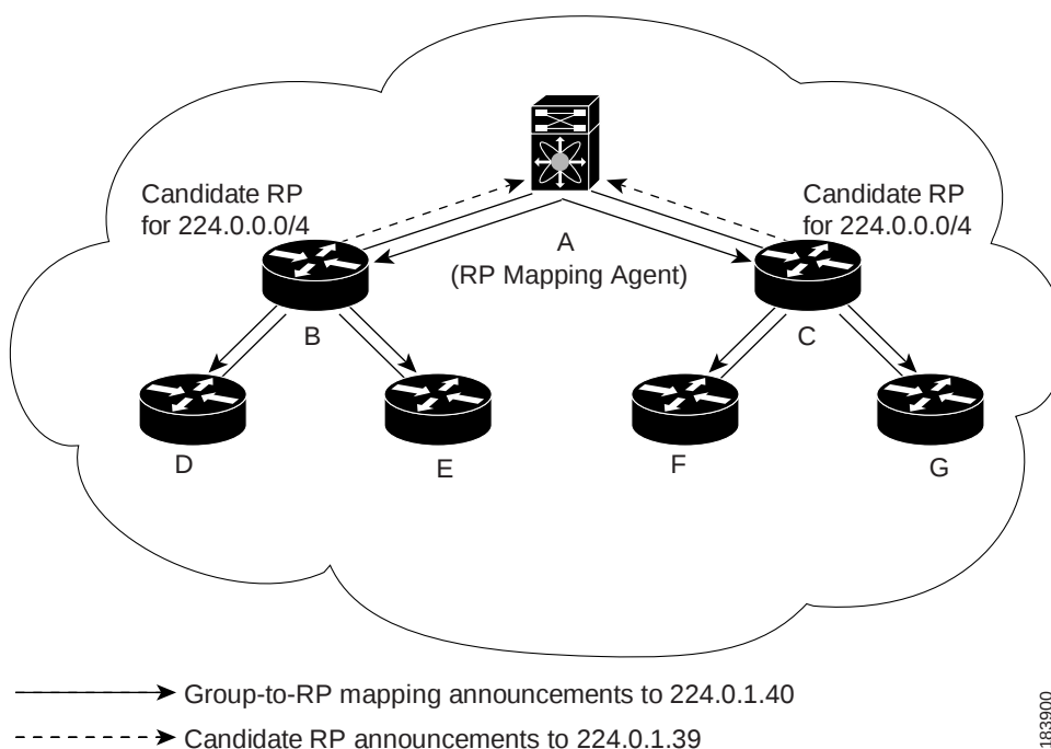
Figure 3-2 Auto-RP Mechanism
