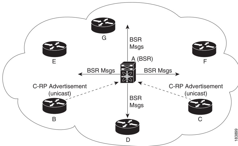
Figure 4-1 BSR Mechanism
