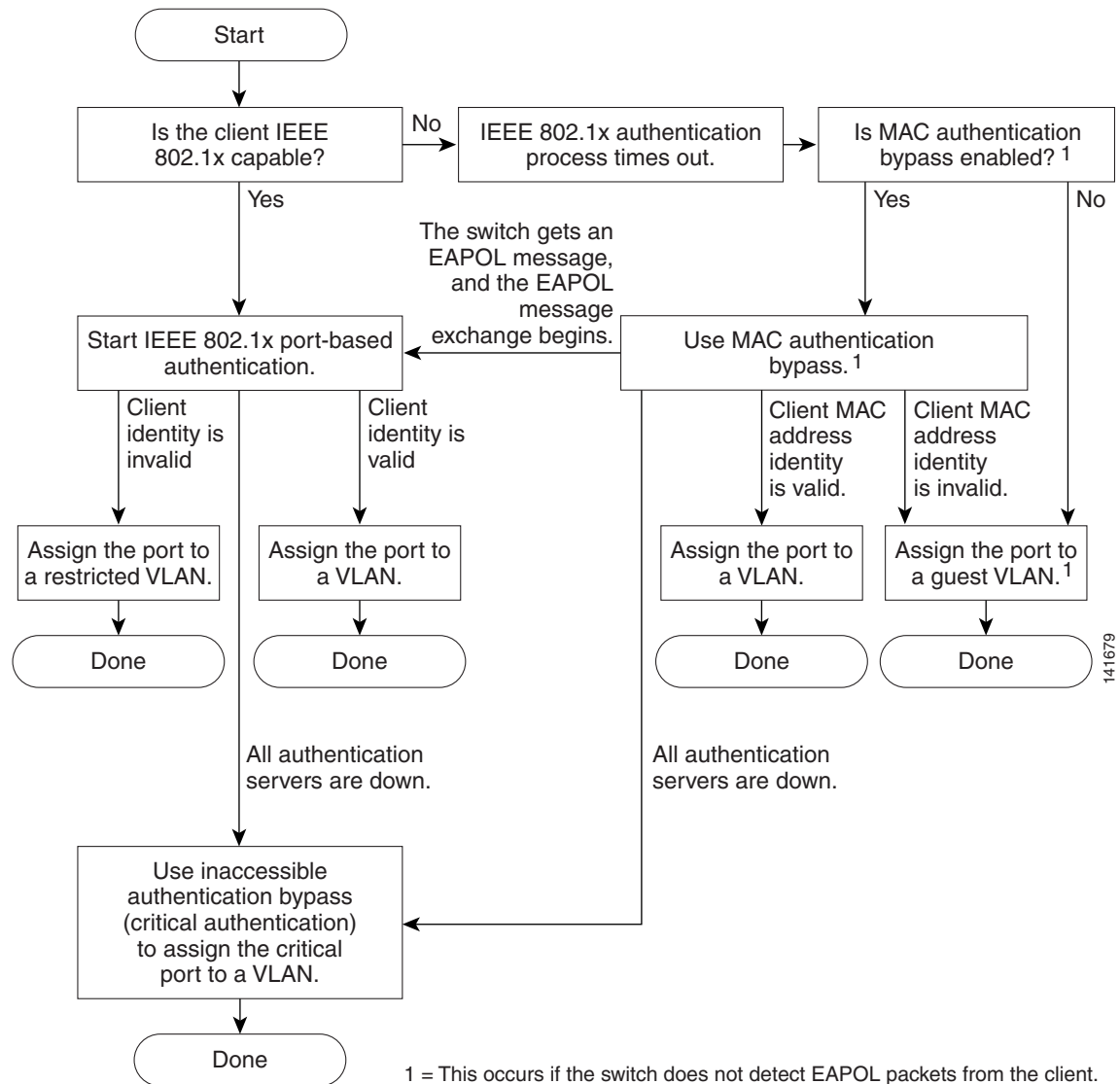
Figure 6-2 Authentication Flowchart
