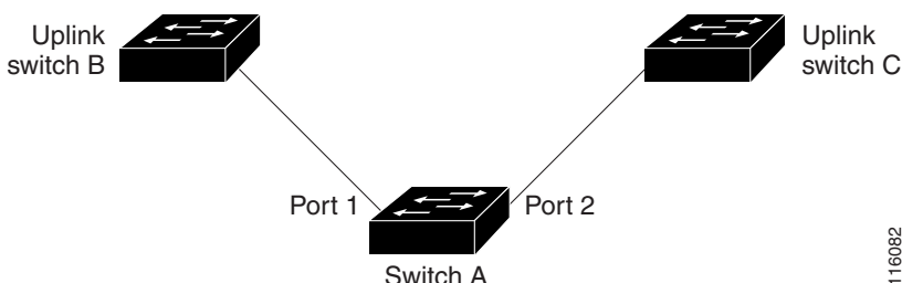
Figure 15-1 Flex Links Configuration Example
