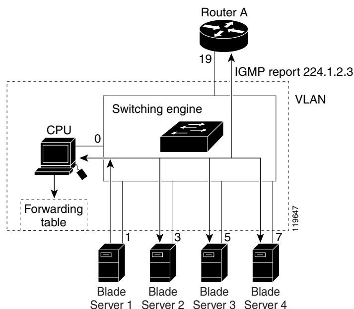
Figure 17-1 Initial IGMP Join Message
