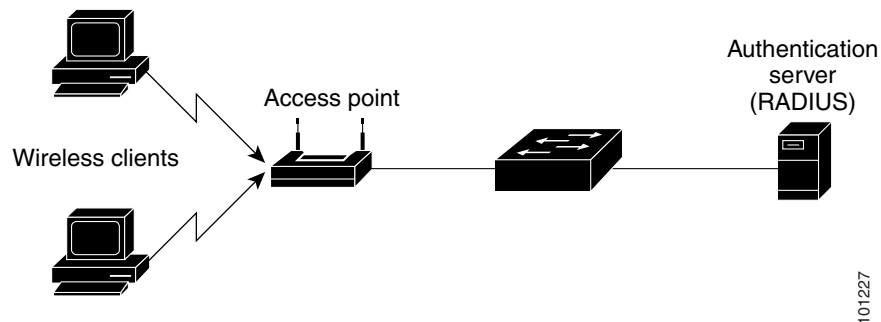
Figure 6-5 Multiple Host Mode Example
