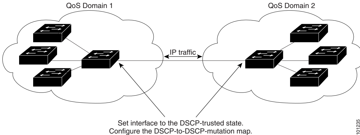
Figure 27-13 DSCP-Trusted State on a Port Bordering Another QoS Domain
