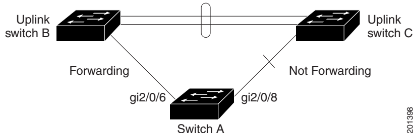
Figure 15-2 VLAN Flex Links Load Balancing Configuration Example
