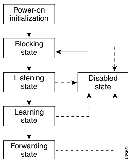
Figure 12-1 Spanning-Tree Interface States
