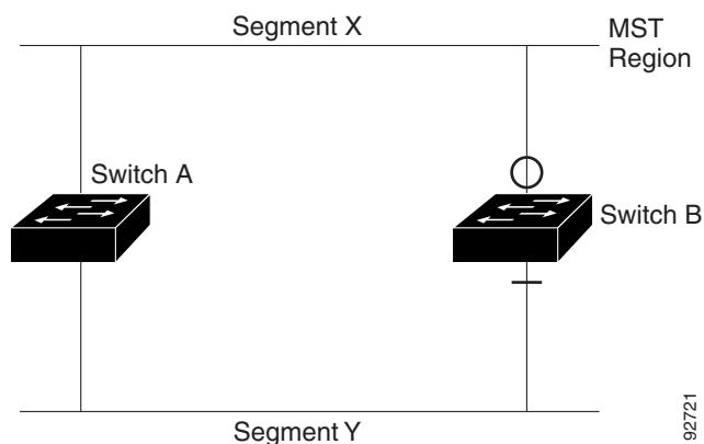
Figure 13-2 Standard and Prestandard Switch Interoperation
