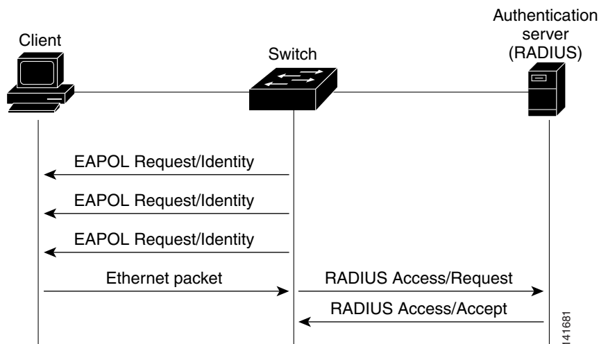
Figure 6-4 Message Exchange During MAC Authentication Bypass
