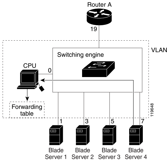
Figure 17-2 Second Host Joining a Multicast Group
