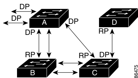
Figure 12-2 Spanning-Tree Topology
