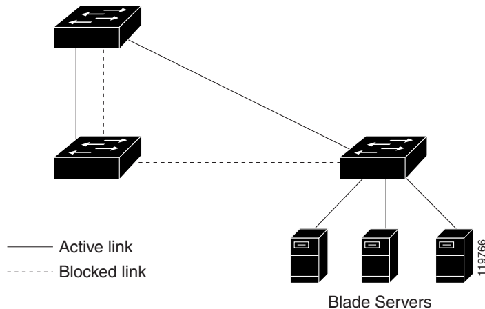
Figure 12-3 Spanning Tree and Redundant Connectivity
