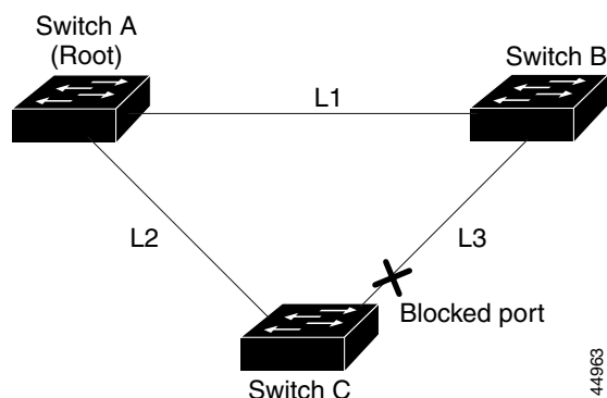
Figure 14-5 BackboneFast Example Before Indirect Link Failure
