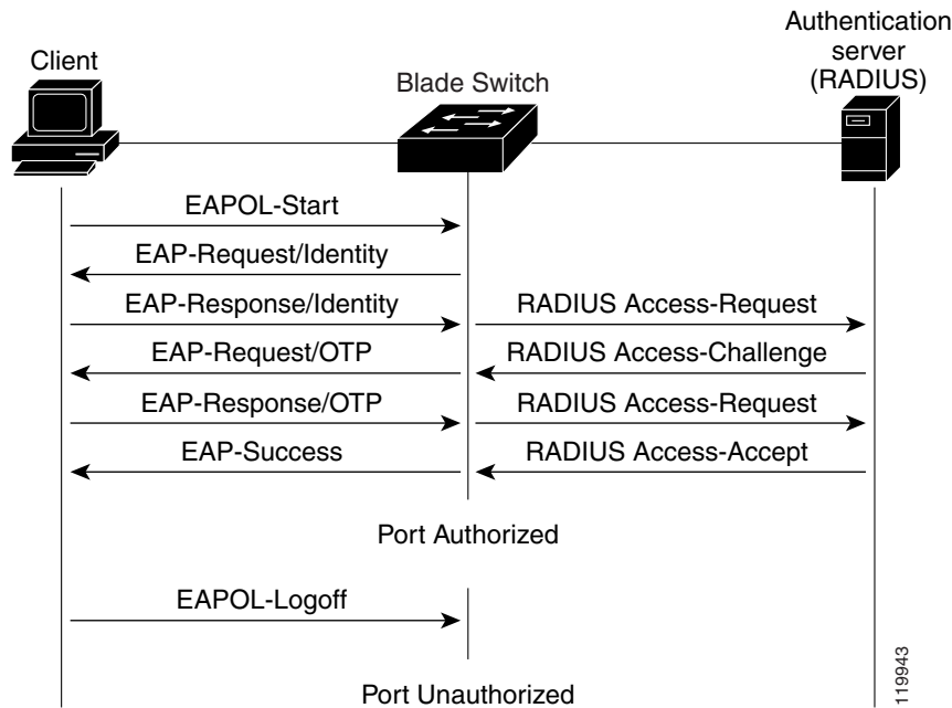
Figure 6-3 Message Exchange
