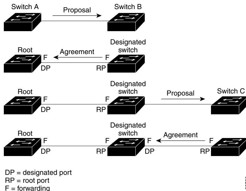
Figure 13-4 Proposal and Agreement Handshaking for Rapid Convergence
