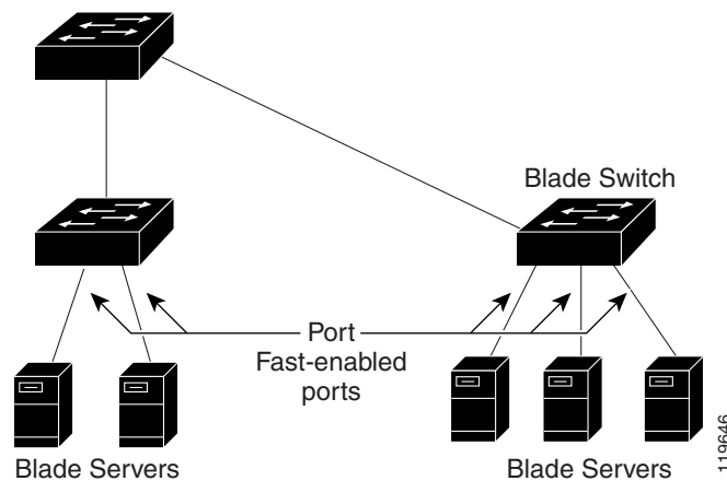
Figure 14-1 Port Fast-Enabled Interfaces
