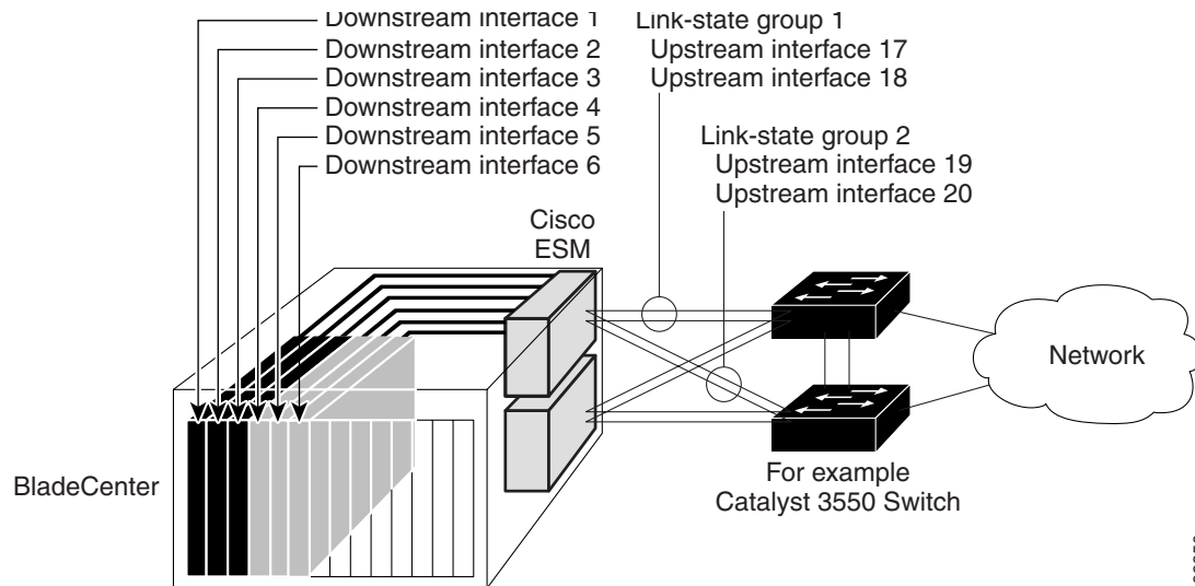
Figure 28-4 Typical Layer 2 Trunk Failover Configuration
