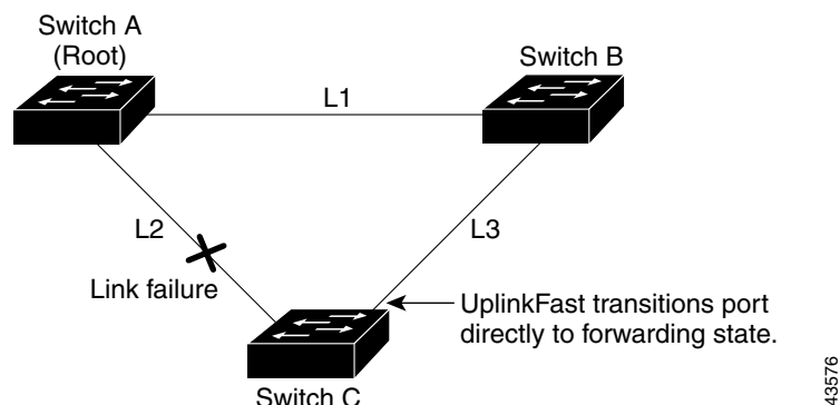
Figure 14-4 UplinkFast Example After Direct Link Failure
