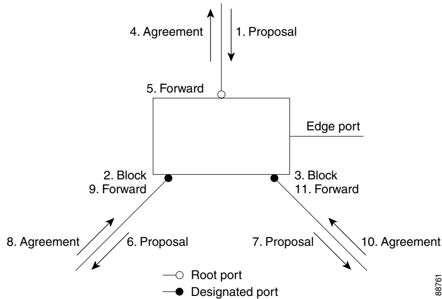
Figure 13-5 Sequence of Events During Rapid Convergence
