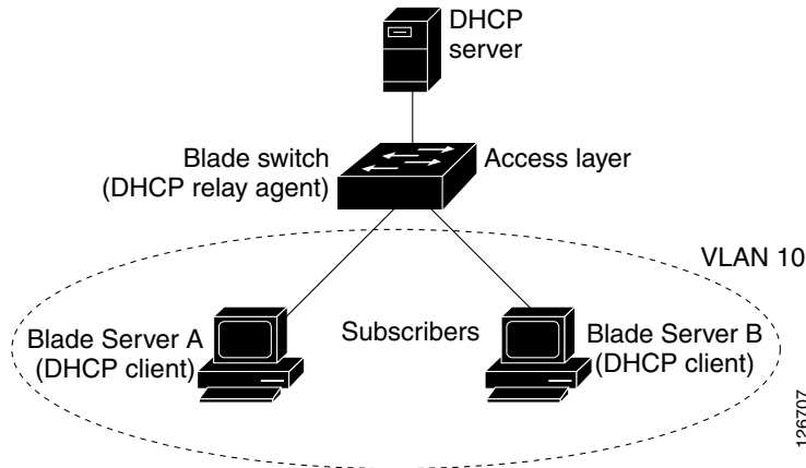
Figure 16-1 DHCP Relay Agent in a Metropolitan Ethernet Network
