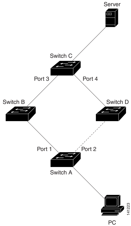
Figure 15-3 MAC Address-Table Move Update Example
