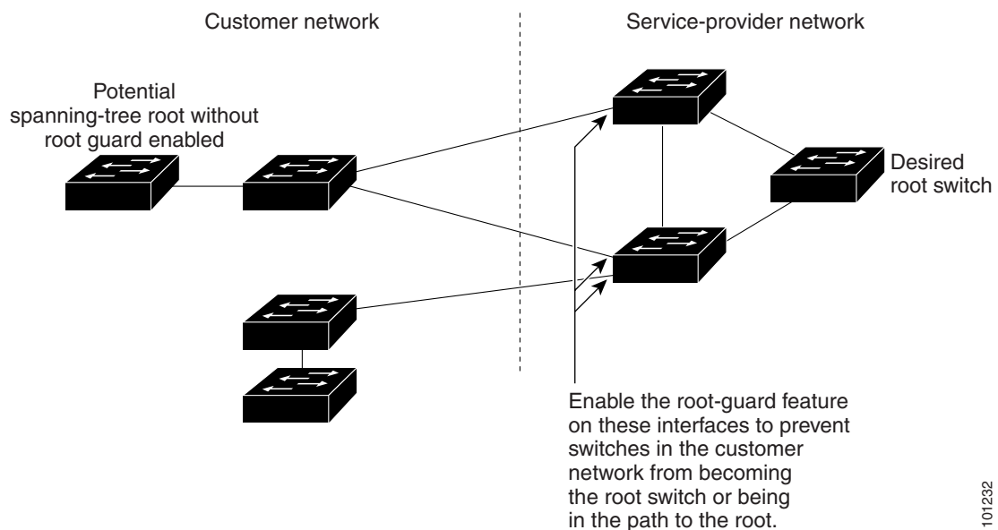
Figure 14-8 Root Guard in a Service-Provider Network
