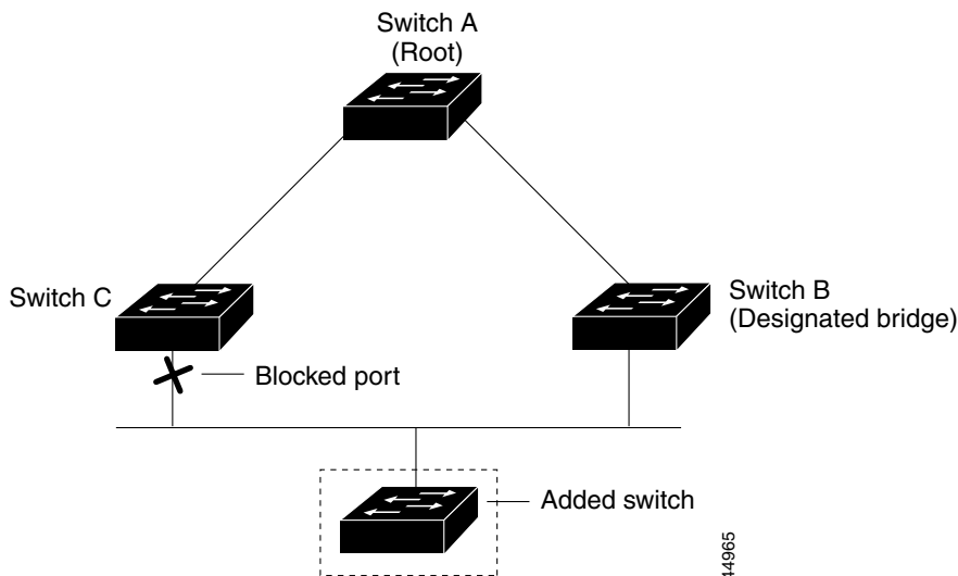
Figure 14-7 Adding a Switch in a Shared-Medium Topology
