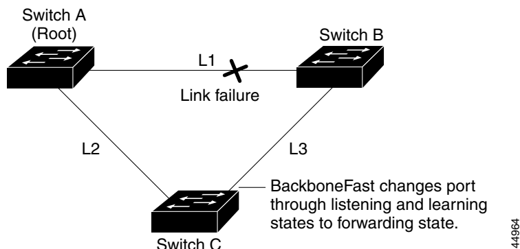
Figure 14-6 BackboneFast Example After Indirect Link Failure
