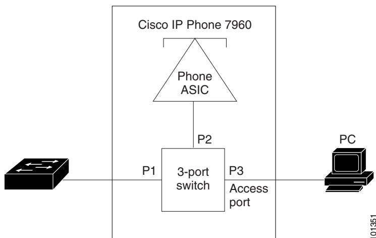
Figure 11-1 Cisco 7960 IP Phone Connected to a Switch
