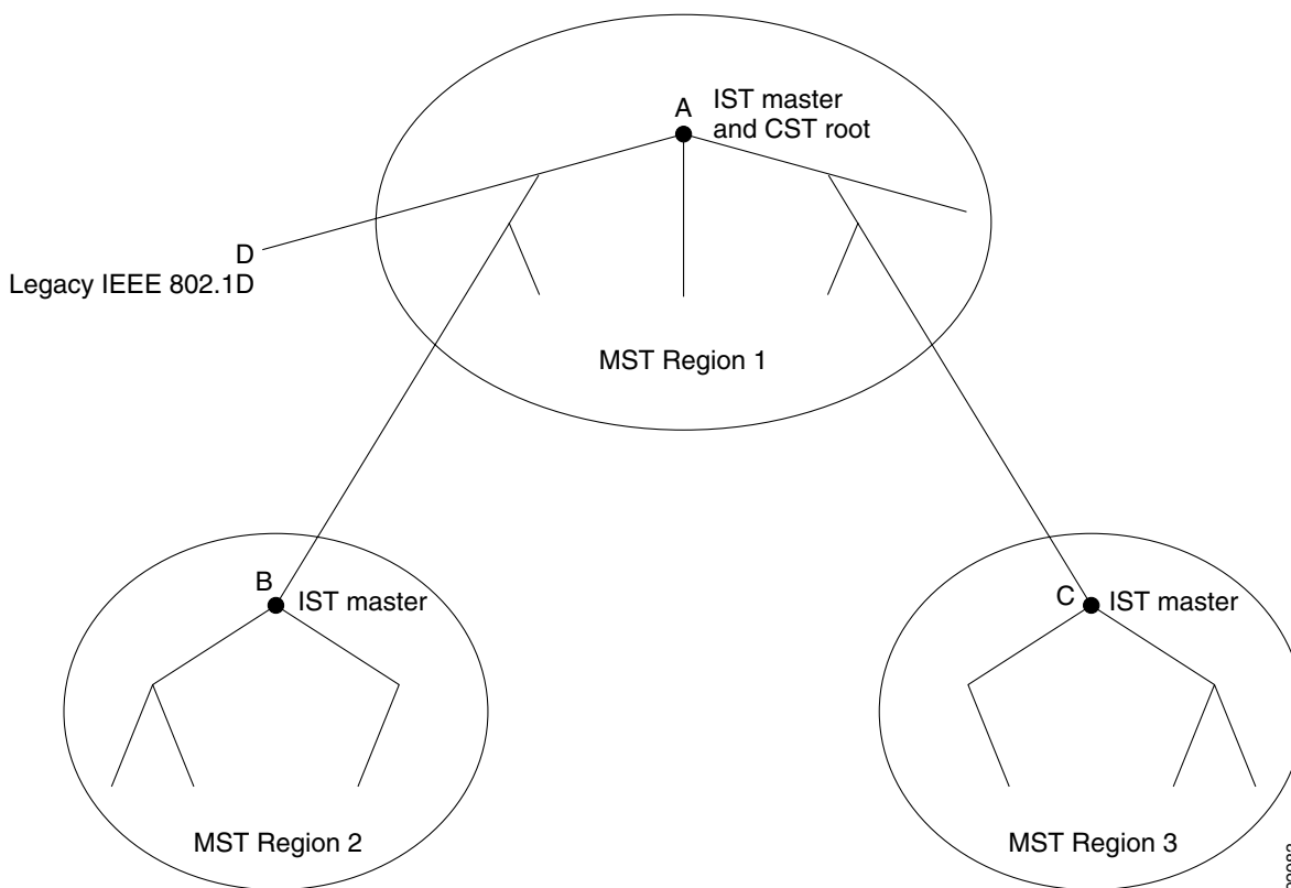
Figure 13-1 MST Regions, CIST Masters, and CST Root
