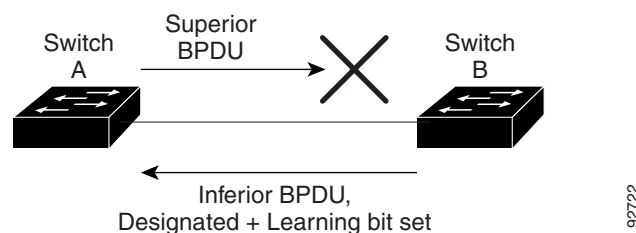
Figure 13-3 Detecting Unidirectional Link Failure
