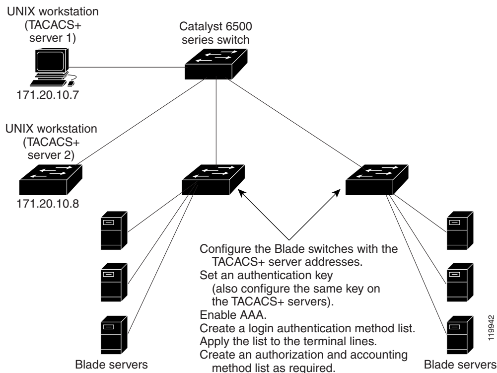
Figure 5-1 Typical TACACS+ Network Configuration
