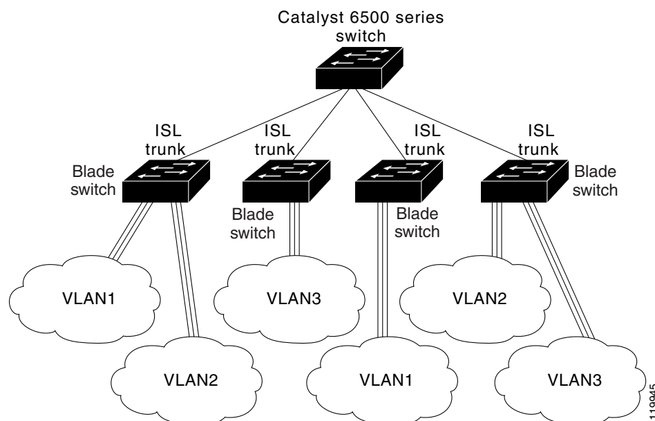
Figure 9-2 Blade Switches in an ISL Trunking Environment
