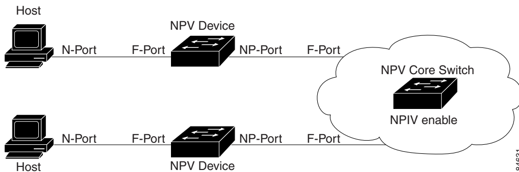
Figure 21-2 Cisco NPV Configuration–Interface View
