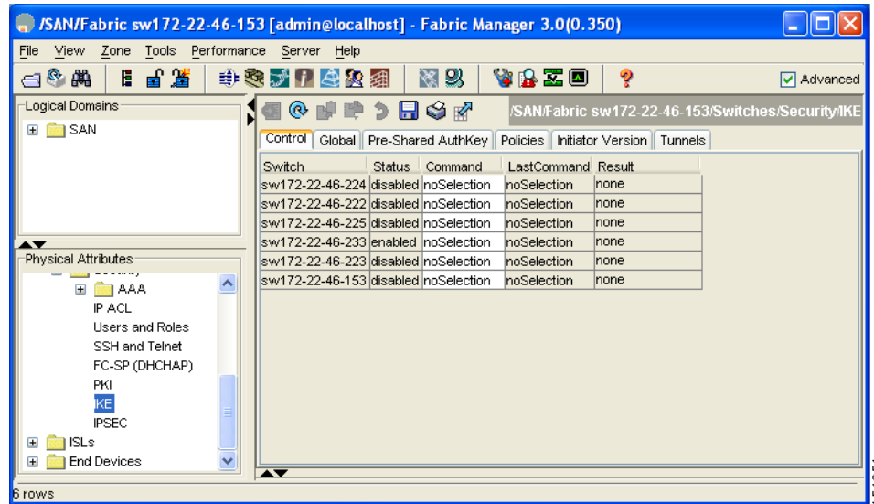
Figure 35-13 IKE Configuration
