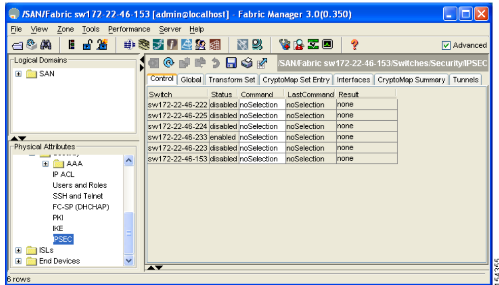
Figure 35-19 IPsec Configuration
