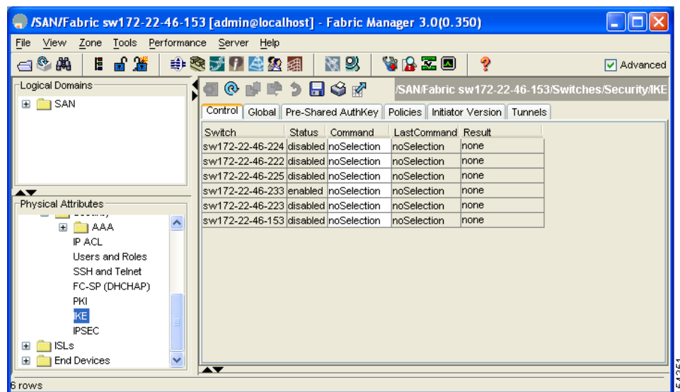
Figure 35-15 IKE Configuration
