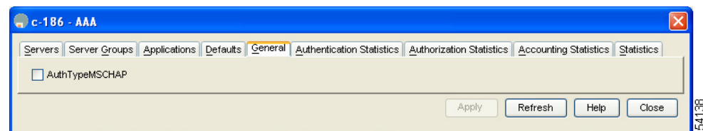
Figure 32-9 MSCHAP Configuration
