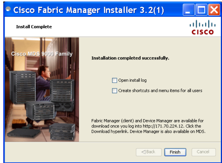
Figure 2-11 Install Complete
