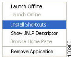
Figure 2-18 Shortcut Menu
