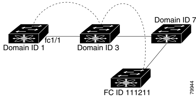
Figure 25-4 Fibre Channel Routes
