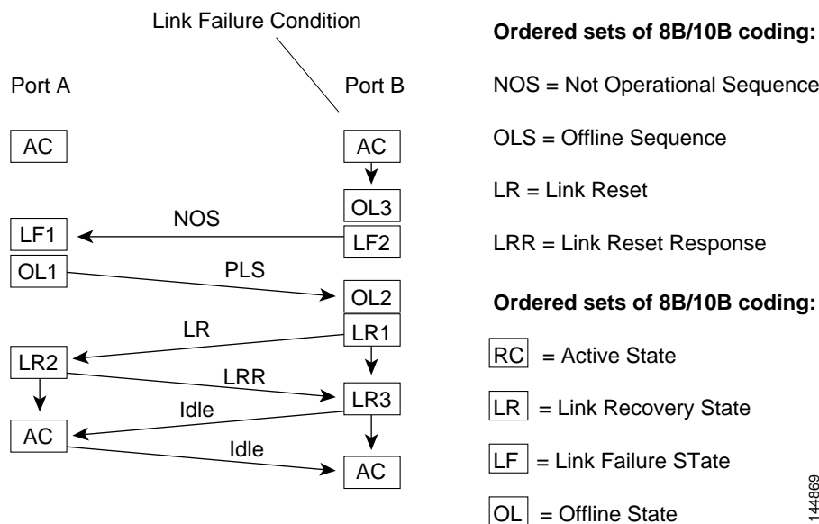
Figure 6-4 Link Initialization Flow
