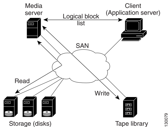
Figure 41-1 Example Configuration with Media Server as Data Mover
