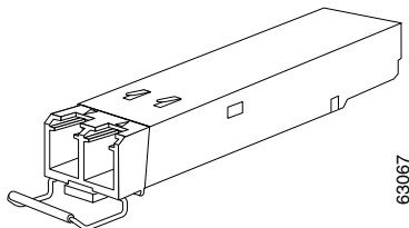
Figure 3-3 SFP Transceiver with Bale-Clasp Latch
