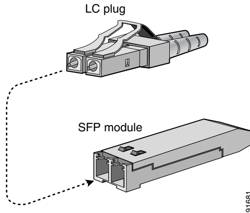
Figure 3-5 Connecting the LC-Type Cable to a Fibre Channel Port
