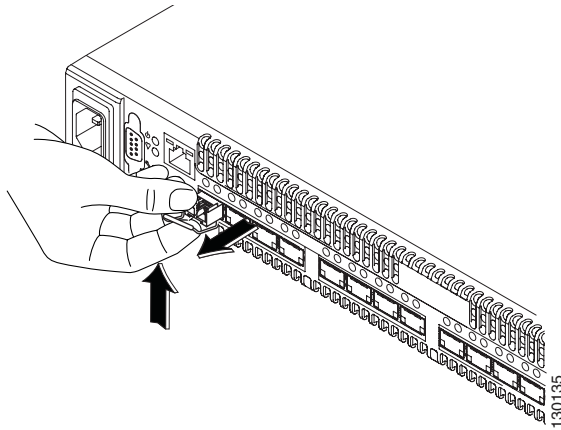
Figure 3-4 Alternate Removal Method for Bale Clasp SFP Transceivers
