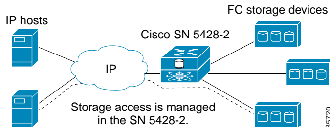
Figure 1 SCSI Routing
